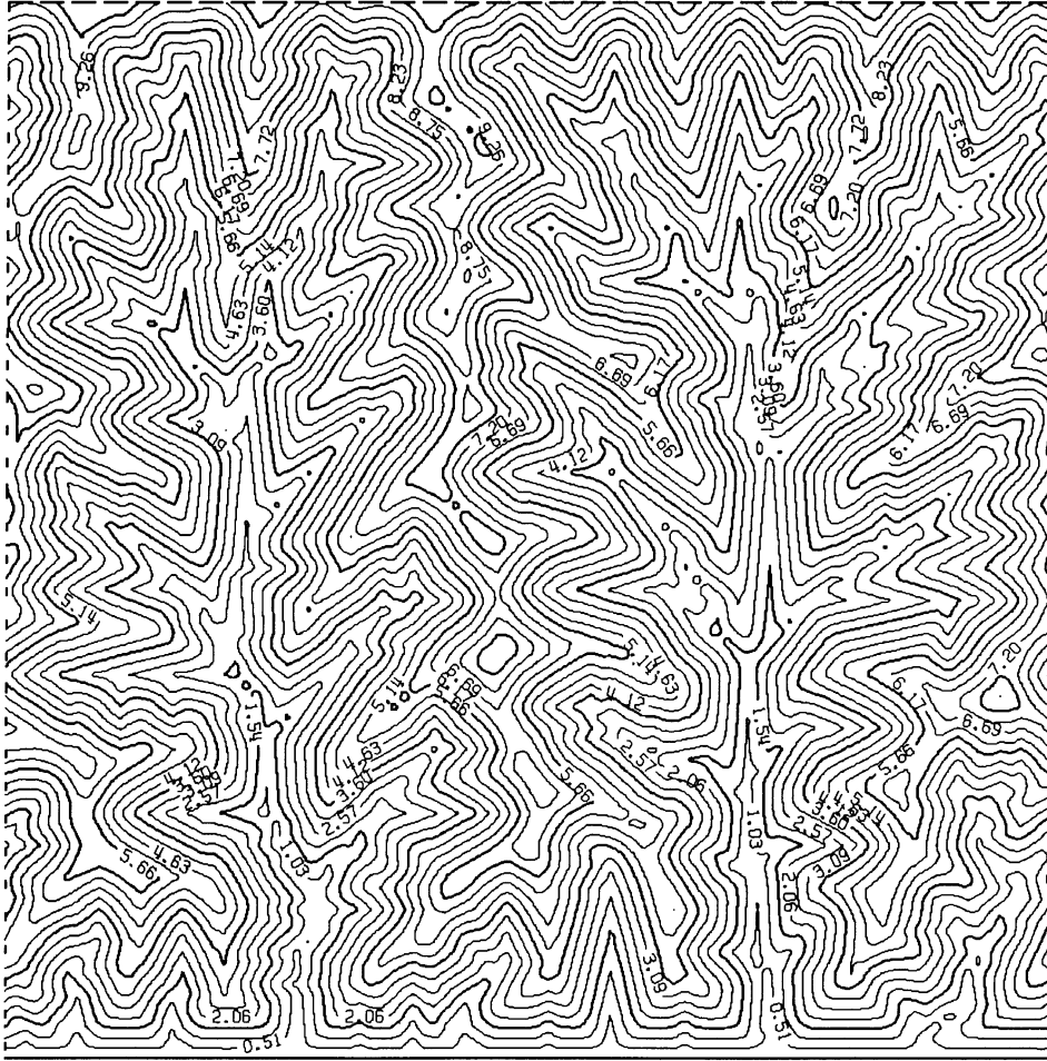
Figure 2. A simulated steady-state drainage basin with maximum slope angles close to the threshold of stability and linear slope profiles. Simulation parameters are K_s = 0.1 , S_t = 0.6 , K_t K_z = 1.0 , X = 500 , \tau_c = 0 , g = 0.3 , h = 0.7 , k_f = 0.5 , a = 3 ; erosion rate, E = -1.0 . The simulation matrix size is 100 \times 100 cells of unity size. Contour interval 0.51, maximum elevation 10.8.
