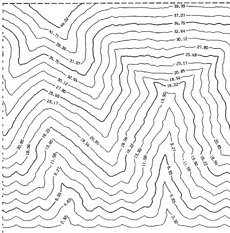
Figure 4. Simulated steady-state topography with simulation parameters as in Figure 2 except that erosion rate, E = 4.0 . Contour interval 2.32, maximum elevation 44.02.
