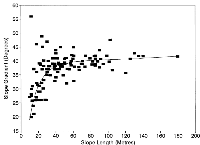
Figure 5. Plot of hillslope gradient versus slope length in Mancos Shale badlands. The short slopes with very high gradients occur on undercut banks along meandering washes.
