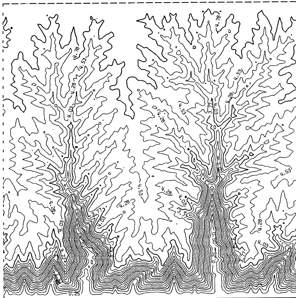
Figure 8. Early stage of dissection of an alluvial surface. Parameters are the same as for Figure 4, except 1/\Psi_c = 0, p = 3, r = 0.5, s = 0.3, t = 3.0 , and K_q K_v = 500 . Downcutting has been stopped after a total vertical erosion of 4.0 units (at a time T_d = 1.0 ). The initial relief on the dissected alluvial surface was 1.5. Present time, T = 2.36 . A small alluvial surface has begun to form adjacent to the lower boundary. Contour interval 0.25, maximum relief 5.3.
